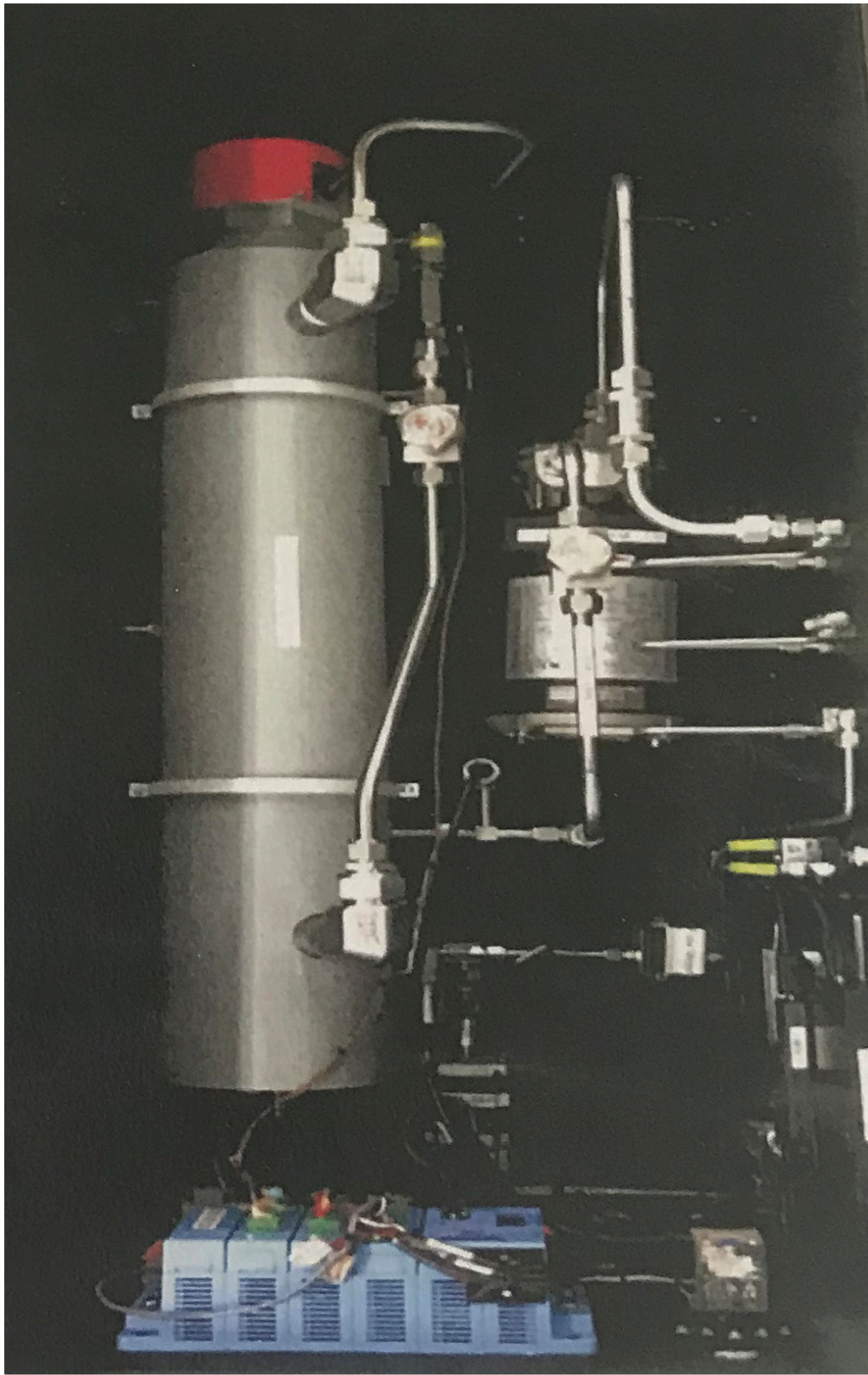
TDSSe (Electric Model) 40" x 20" x 20" Daily Output - 300 Gallons per Day (GPD) Weight - 90 lbs or 41 kg
