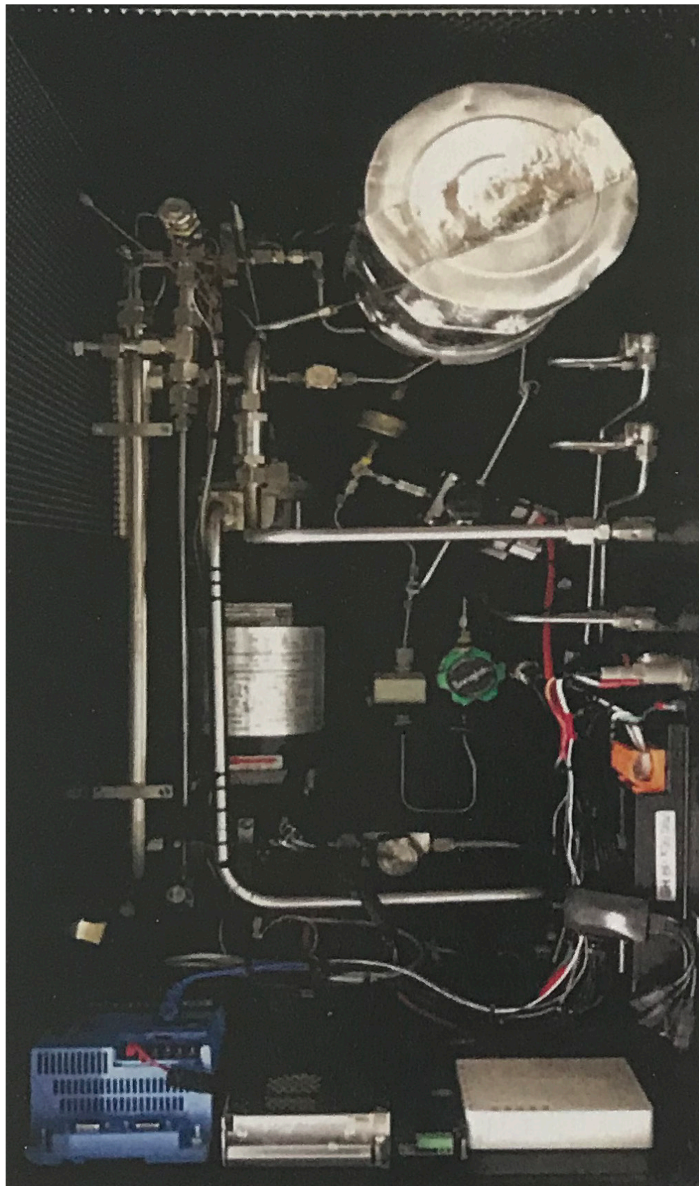
TDSSg (Gas Model) 36" x 18" x 18" Daily Output - 500 Gallons per Day (GPD) Weight - 60 lbs or 27 kg
